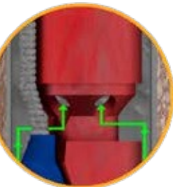
Intake ESP (2 stage)
